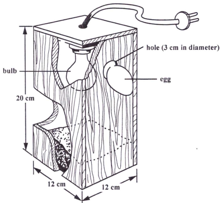
Figure 1. Equipment used in rearing layer birds
